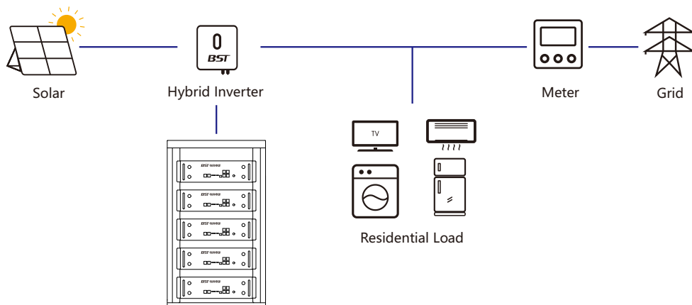
Up to 15 Batteries in Parallel
